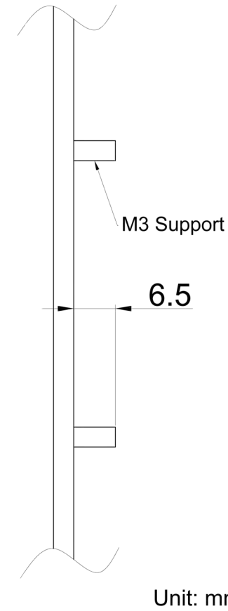
SIDE VIEW
