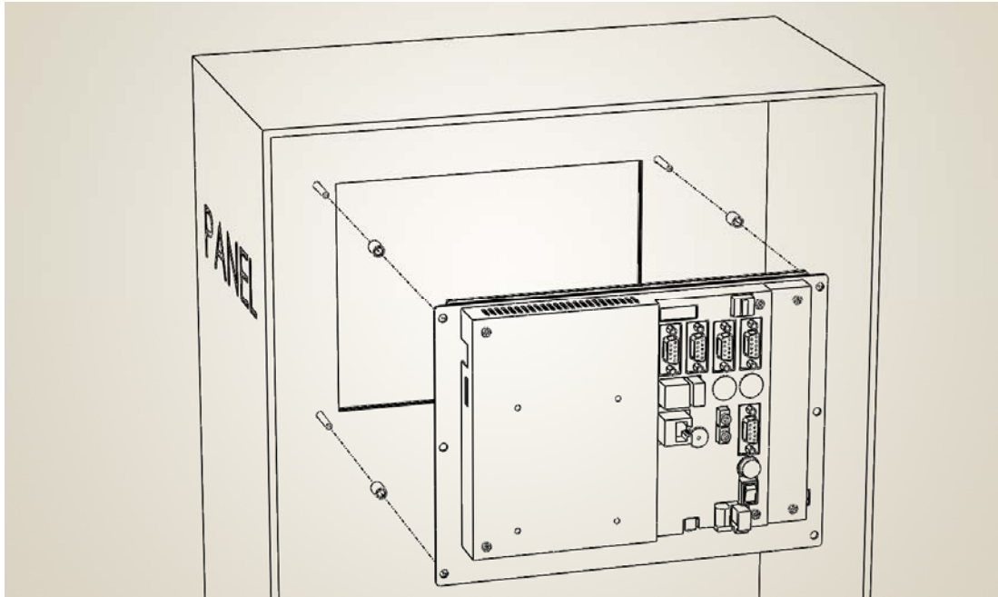
[Figure 5] Before, Spacer and Main Body Mounting (Back Panel)
