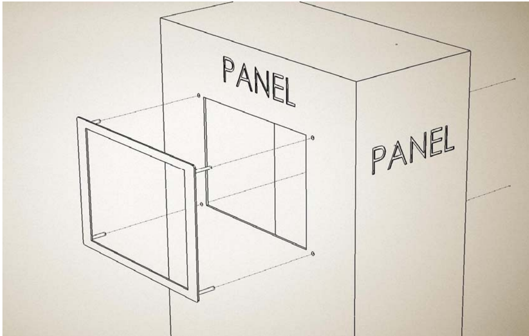
[Figure 3] Before, Bezel Mounting (Front Panel)
