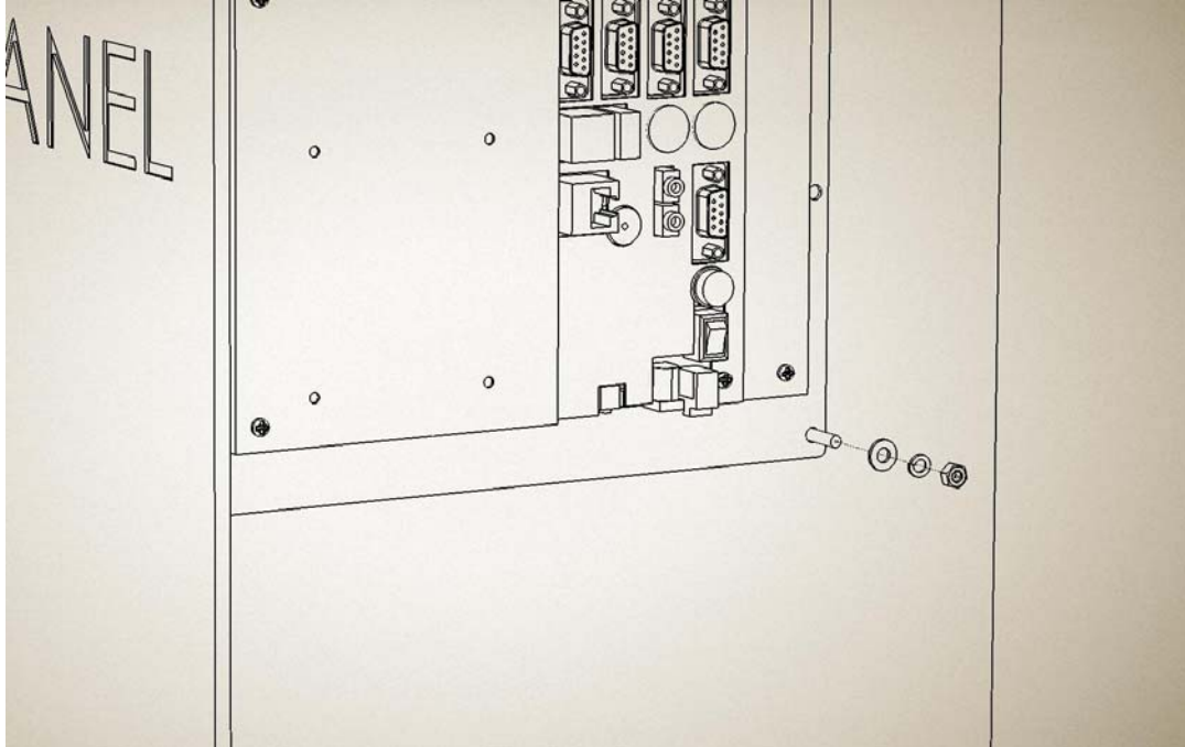
[Figure 7] Before, Washer and Nut Assy. (Back Panel)
