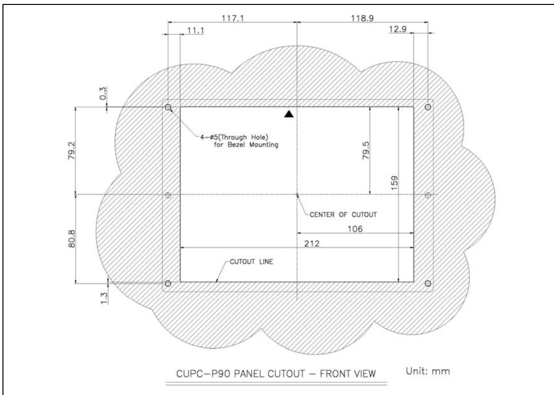
[Figure 2] Panel Cutout Drawing
