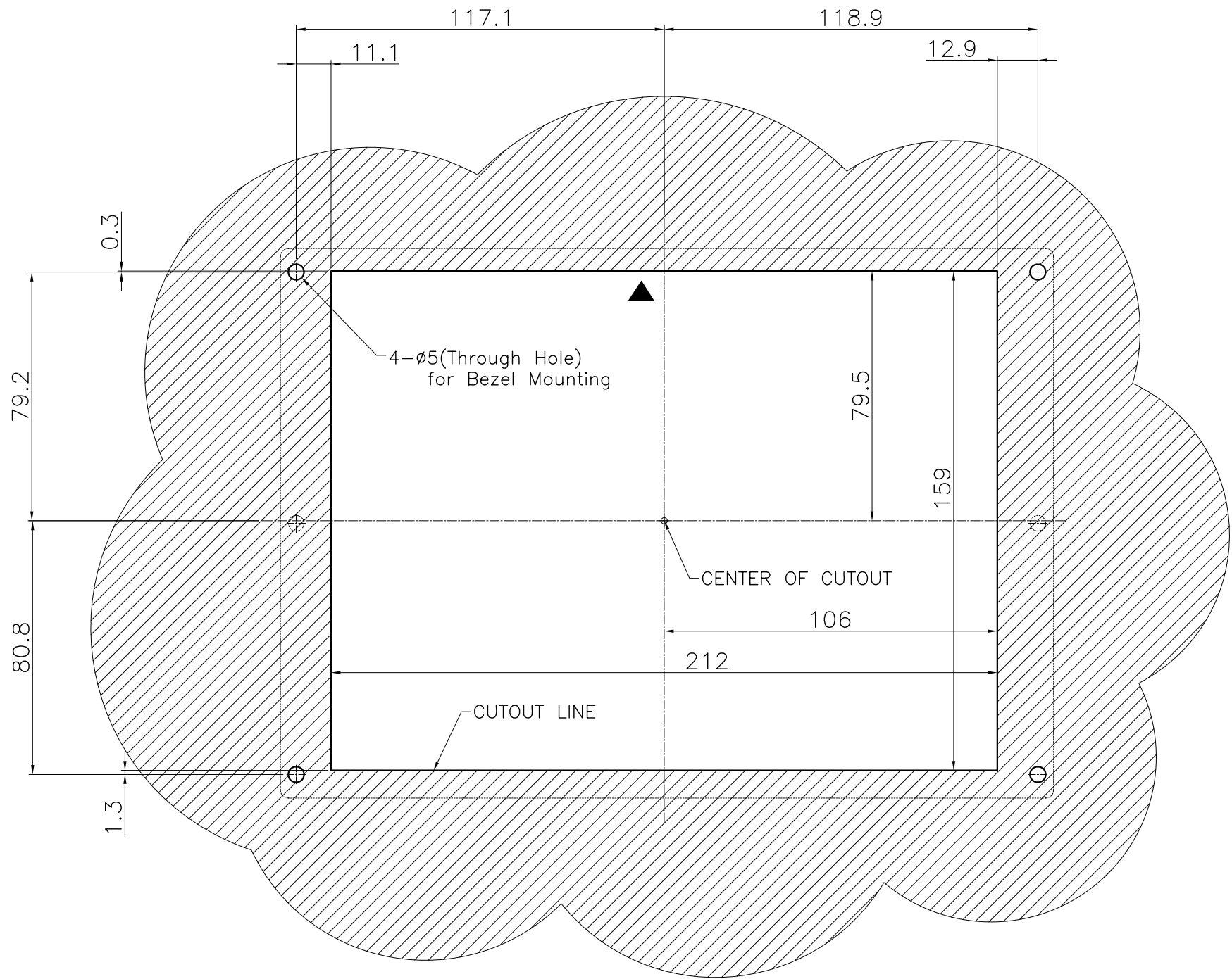
CUPC-P90 PANEL CUTOUT – FRONT VIEW
