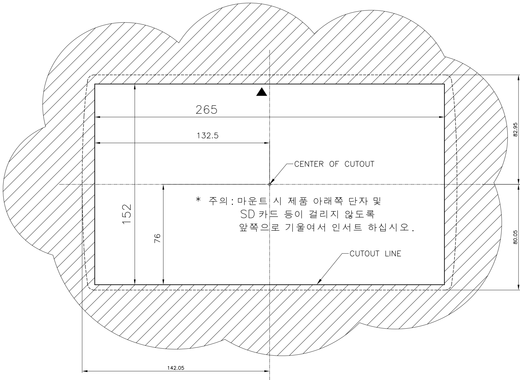
CUPC-P80 PANEL CUTOUT – BACK VIEW
