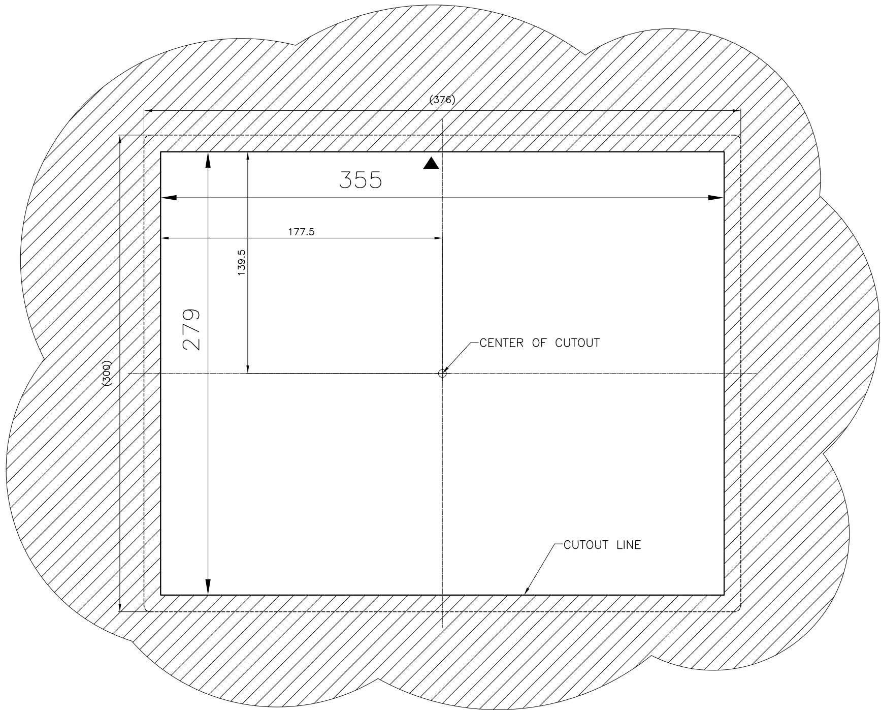
CUPC-P200 PANEL CUTOUT – BACK VIEW
