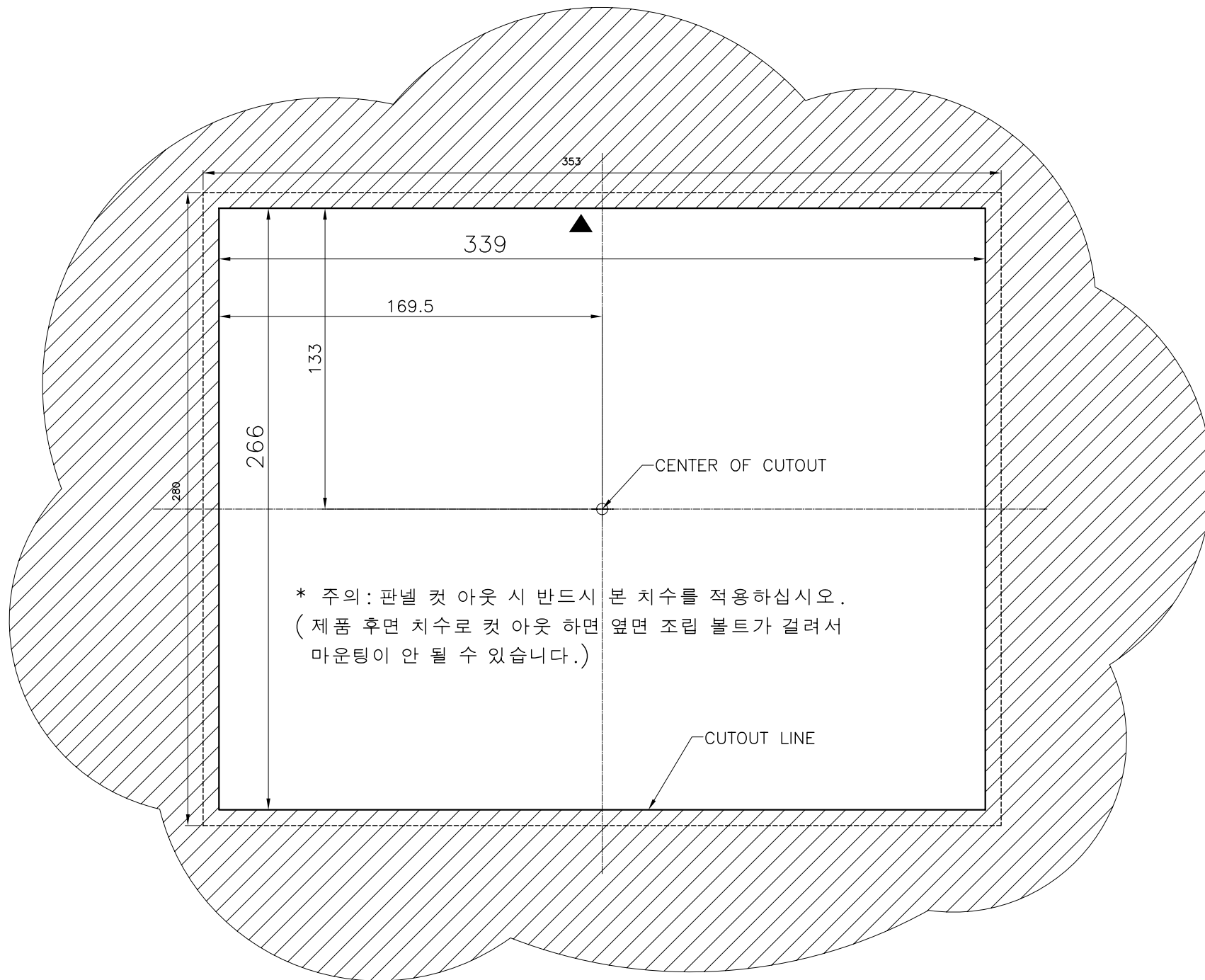
CUPC-P100 PANEL CUTOUT – BACK VIEW
